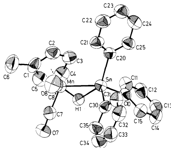
Figure 1. An ORTEP drawing of 1 . Hydrogen atoms at the phenyl rings and the MeCp ligand are omitted for clarity.
